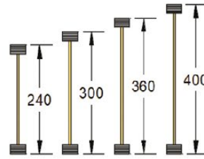
58x35 mm LVL Flange 9.5 mm OSB Web
